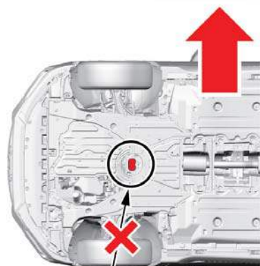
FRONT LIFT POINT
